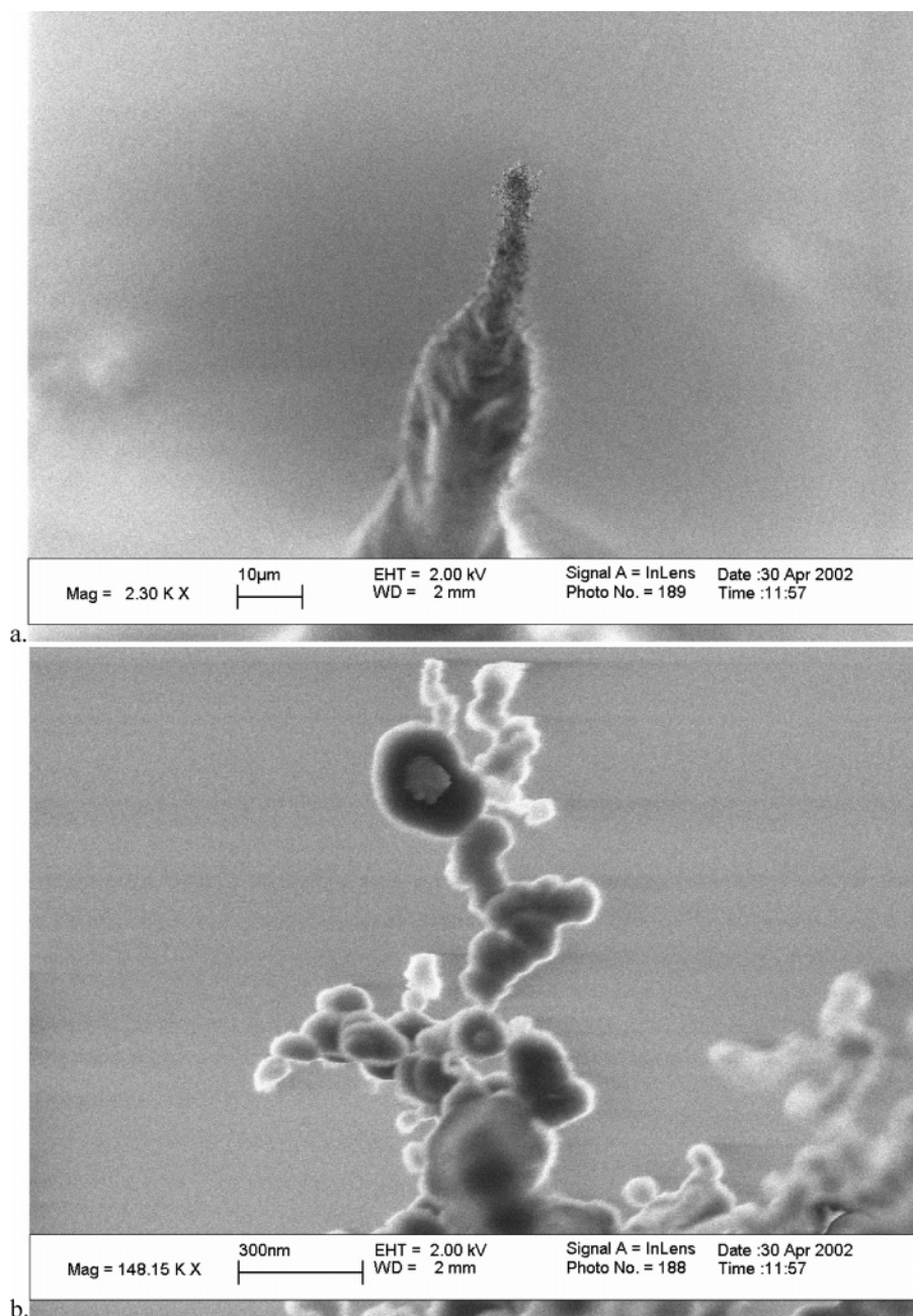
Figure 2. SEM images of the \text{Al/C}_8\text{F}_{17}\text{COOH} composite at (a) 2K and (b) 148K magnification.
