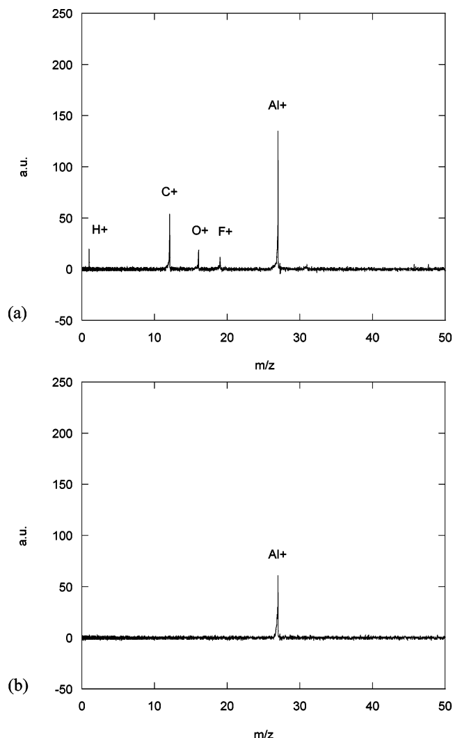
Figure 11. Typical mass spectra for (a) \text{Al/C}_{13}\text{F}_{27}\text{COOH} particles and (b) pure aluminum nanoparticles measured with SPMS at 25 °C.
