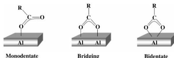
Figure 8. Three proposed structures for carboxylate binding to Al surface. In the monodentate geometry only one oxygen atom is bonded to the aluminum surface. For the bidentate coordination, the oxygen atoms are both bonded to the same aluminum atom. In the bridge-bonded configuration, the oxygen atoms are identical but on different aluminum atoms.
